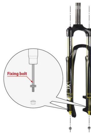
Figure: Multiple fixing bolt versions (Right and Left Sides)
